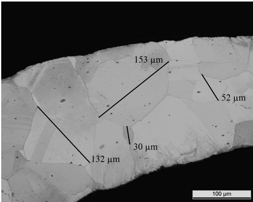
Figure 6: Metallographic section of the garland of the horn by Millereau (Appendix, no. 34), etched by Klemm. Alpha brass with lead inclusions (dark), secondary recrystallized grain structure with twins (parallel lines), and strain lines on the surface are visible.
